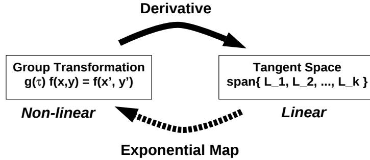
Figure 1: The relationship between the Lie group and its tangent space (Lie algebra) is due to the exponential map, which maps an element in the tangent space onto an element of the group in the neighborhood of the identity.
