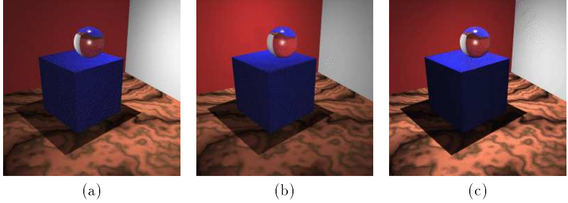
Figure 28: Images of a scene illuminated by a directional spot light. The angular radiance distribution of the light source is a fifth degree polynomial. Each of the images were re-rendered by linearly combining a set of 12 basis images. The left and middle images show the scene re-rendered with the spot light pointed in different directions. The right image shows the scene re-rendered with two spot lights in the same position, but pointing in different directions.
